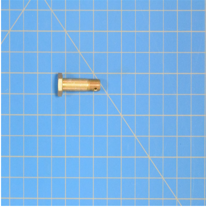
NAS1005-14D - Bolt
