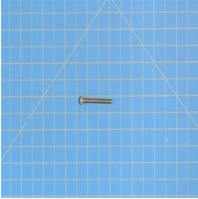
MS51957-125 - Screw
