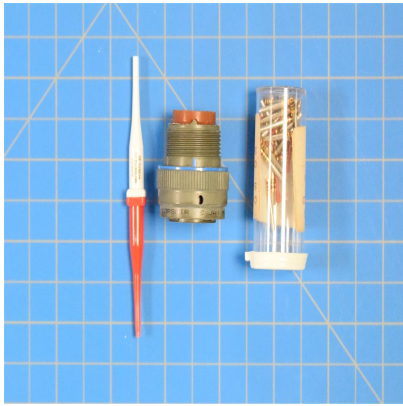
MS3476W16-26S - Connector
