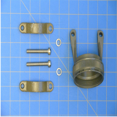
M85049/52-1-24W - Backshell, Circular Connector, Straight
