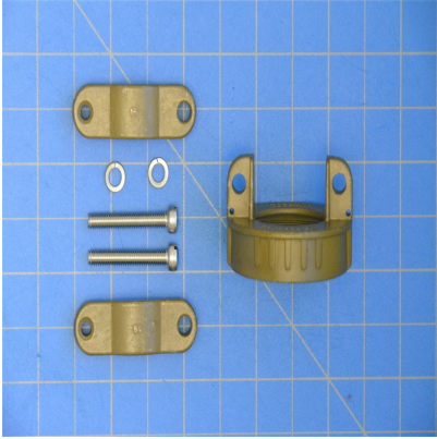
M85049/41-16A - Backshell, Circular Connector, Size 24
